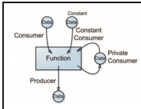
Figure 8: Classification of data dependencies
