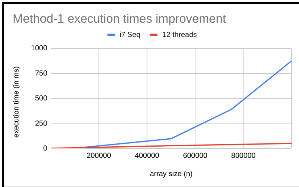
Figure 13 : Results of Method-1 on i7 9th gen
